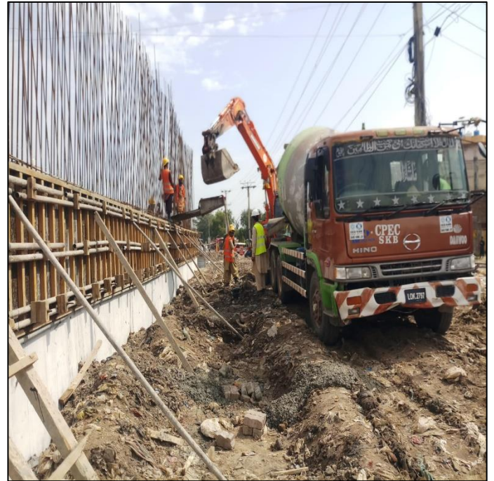
Picture 70: Pouring of Retaining Wall Concrete is in Progress
