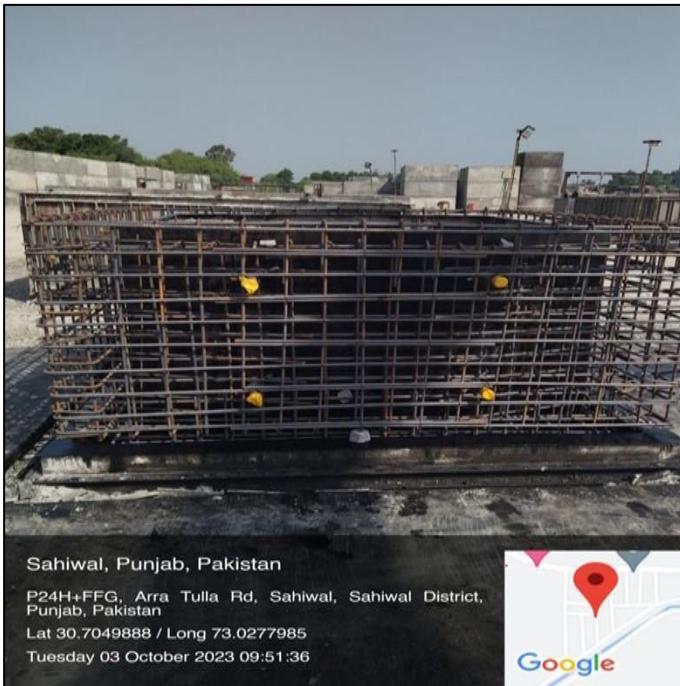
Picture 18: Steel cage of 10 x 8.25ft conduit
