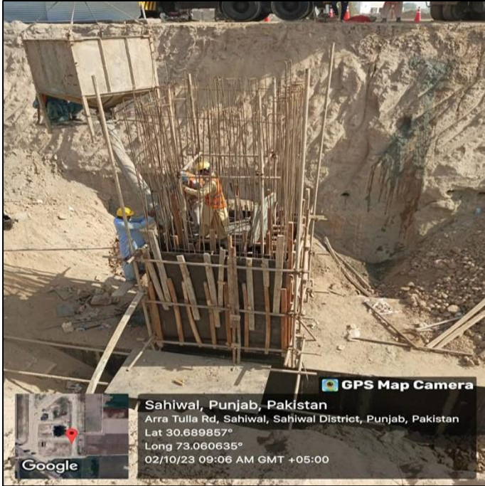
Picture 20: Concrete Pouring in Manhole walls at Arra Tullah Road
