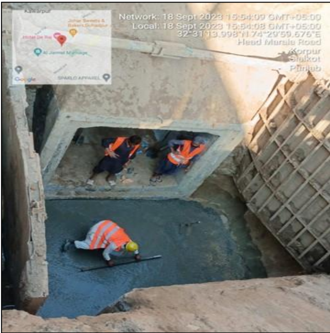
Picture 38: Lean for Manhole 69 in Progress at Marala Road
